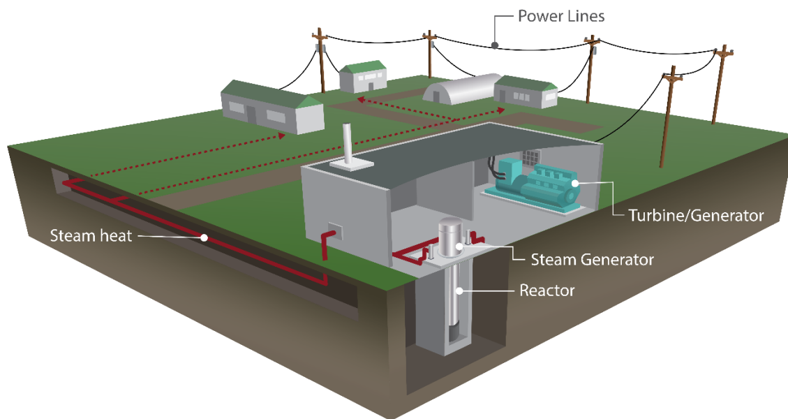
Figure 2.2. An SMR or MNR is designed to be delivered to the site with key components (or in some cases the entire system) packaged in self-contained housing that is often buried below grade. Many of these reactors generate steam which is used to generate power. Heat can be delivered via a steam or hot water district heating system.
