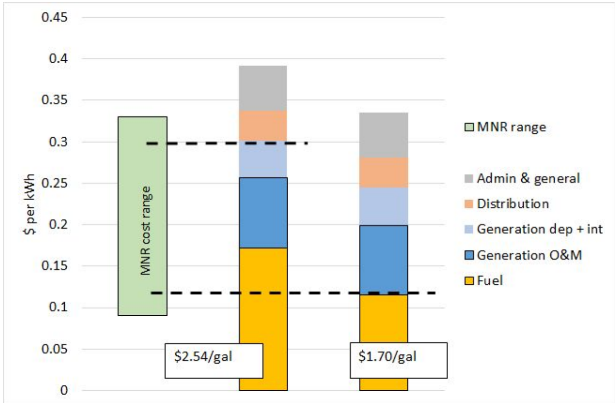
Figure 5.3 Comparison of the cost components of electric service in a representative Alaska hub community, under two different fuel prices, to the potential range of production costs for electricity from an MNR.
