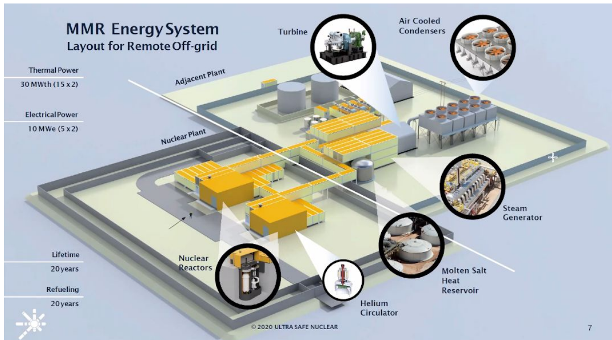
Figure 2.4. A proposed layout for the Ultra Safe Nuclear Corporation Micro Modular Reactor Energy System (MMR), which incorporates two reactors each capable of supporting 5 MW of electric power generation. Other configurations are also possible, including a single unit or multiple units. (Image courtesy of USNC)
